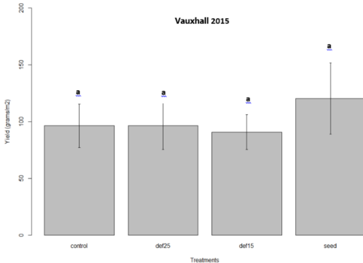
Fig. 3. Yield (g/m 2 ) of canola from the economic threshold small plot study conducted at Lethbridge, Alberta
